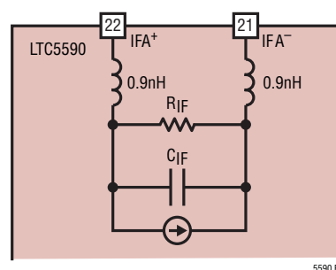
Figure 8. IF Output Small-Signal Model
