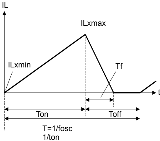
Discontinuous Mode
