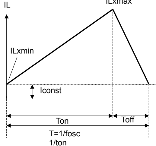
Continuous Mode
