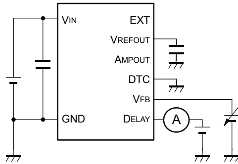
Fig.4 DELAY Pin Charge Current/Discharge Current Test Circuit
