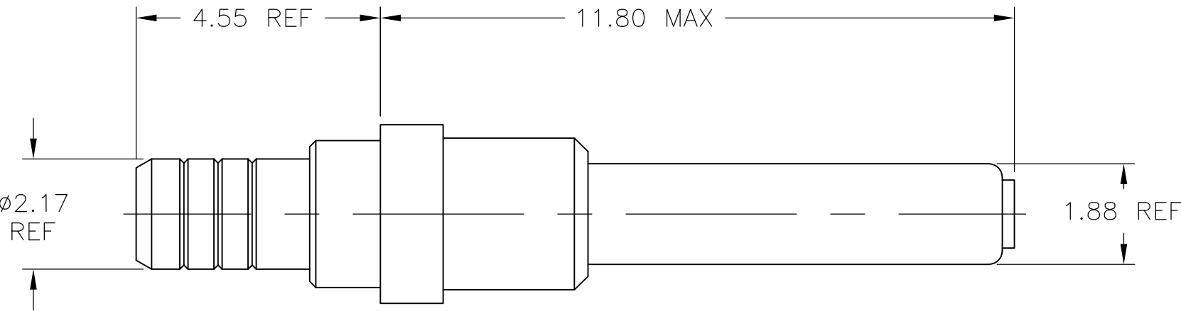
OUTER CONTACT
