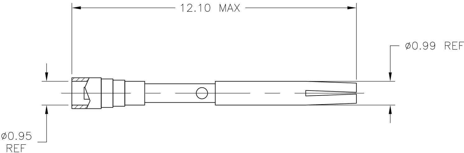
CENTER CONTACT
