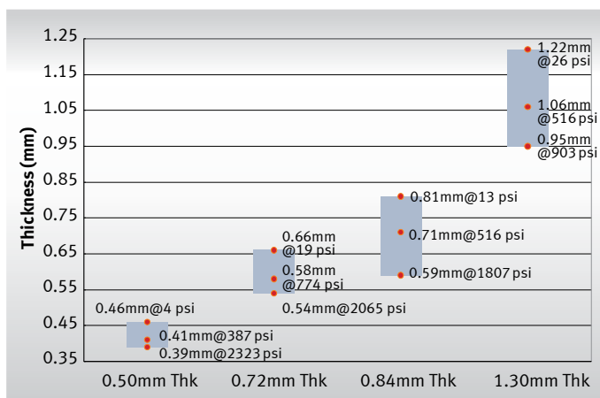
FIGURE 2: RECOMMENDED SERVICE HEIGHTS FOR SMT GS5200 SERIES
