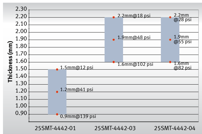
FIGURE 1: RECOMMENDED SERVICE HEIGHTS FOR SMT SUPERSOFT SERIES
