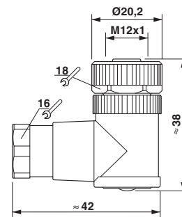
Dimensioned drawing
