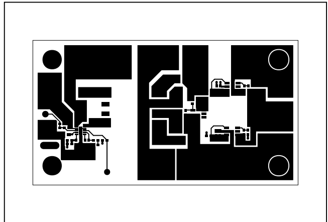
Figure 2. MAX17681 EV Kit PCB Layout—Component Side
