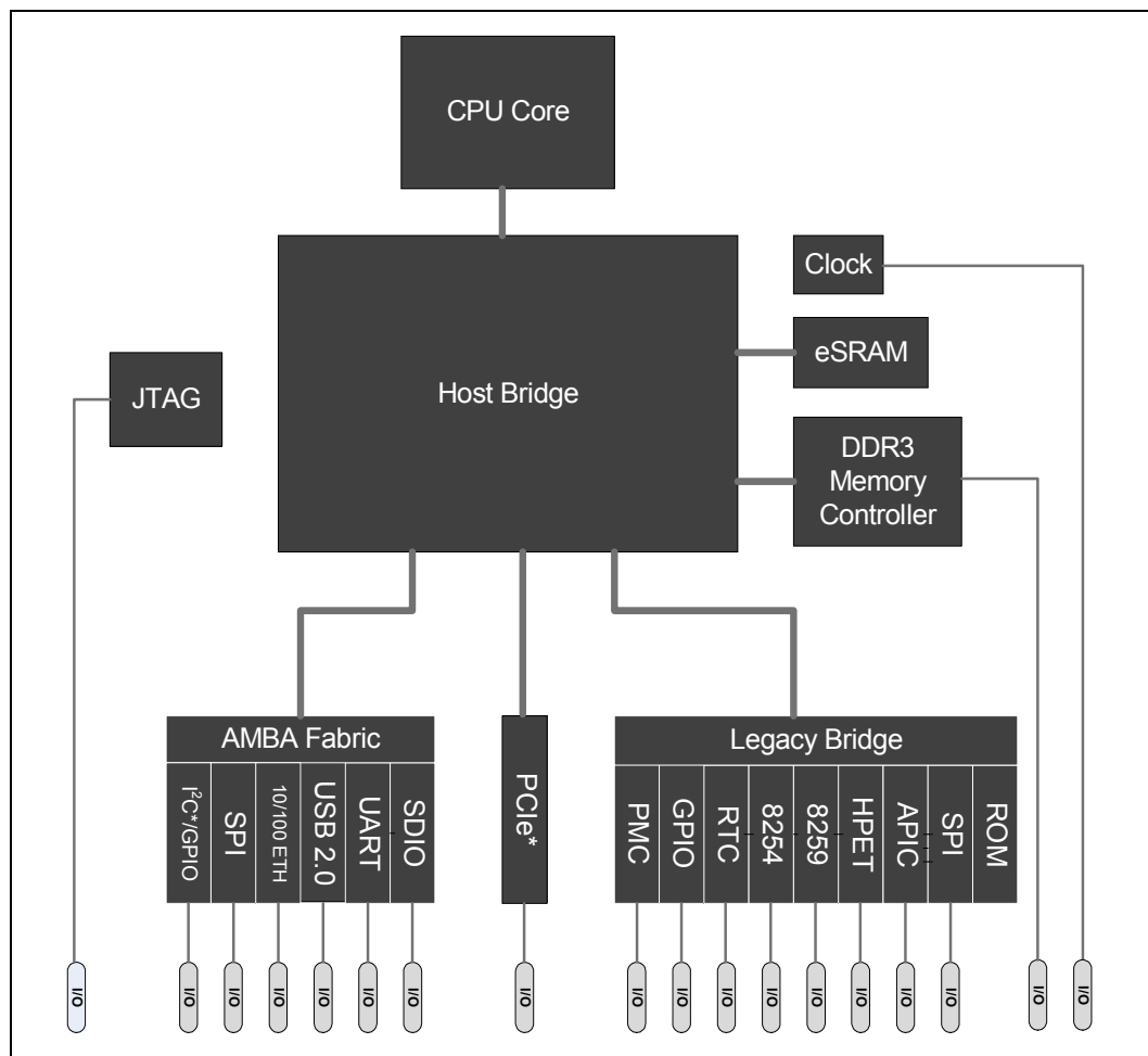
Figure 1. Block Diagram
