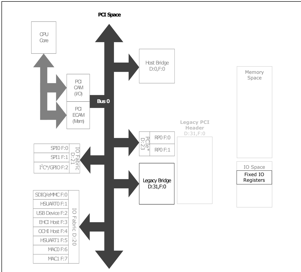
Figure 55. 8259 Register Map
