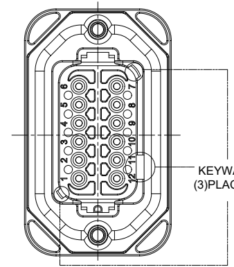
P/N AT15-12PD-BM1X KEY-D CONFIGURATION STANDARD COLOR: BROWN
