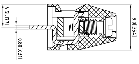
SECTION P-P
