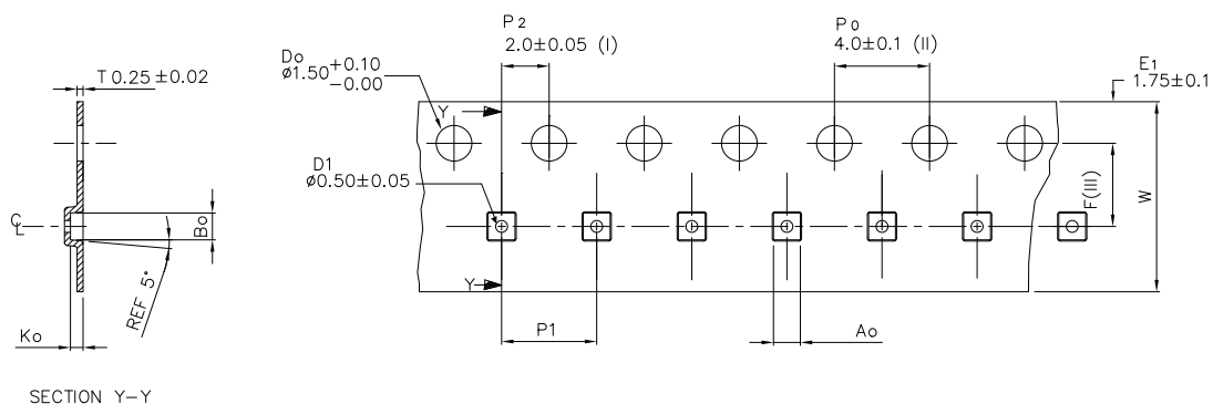
Figure 24. Tape dimensions
