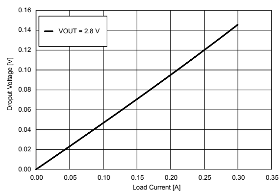
Figure 11. Dropout voltage vs. load current
