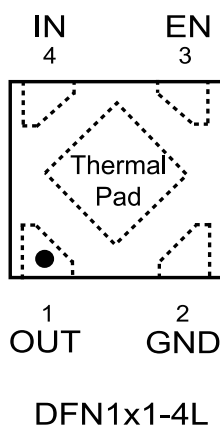
Figure 2. Pin connection (top view)
