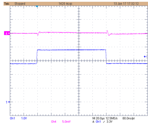
Figure 19. Line transient ( V_{OUT} = 1.8\text{ V} ; I_{OUT} = 10\text{ mA} , t_r = t_f = 1\text{ }\mu\text{s} )
