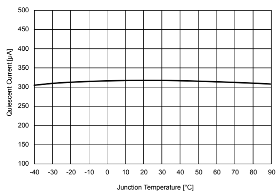
Figure 9. Quiescent current vs. temperature ( I_{OUT} = 300 mA)
