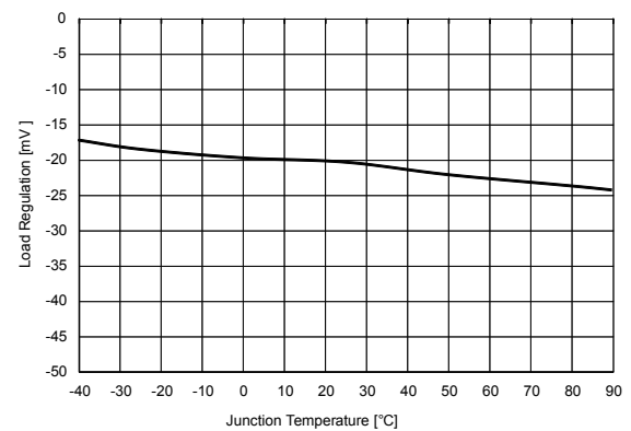
Figure 7. Load regulation vs. temperature ( V_{OUT} = 1.8 V ; I_{OUT} = 0 to 300 mA )
