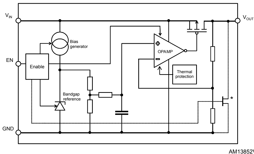
Figure 1. Block diagram
