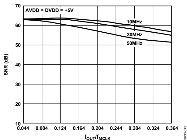
Figure 13. SNR vs. f_{OUT}/f_{MCLK} for Various MCLK Frequencies
