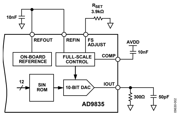
Figure 2. Test Circuit
