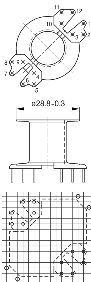
12 pins
