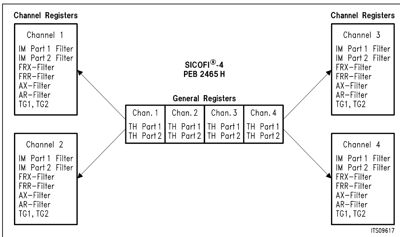
Figure 9 Channel Registers
