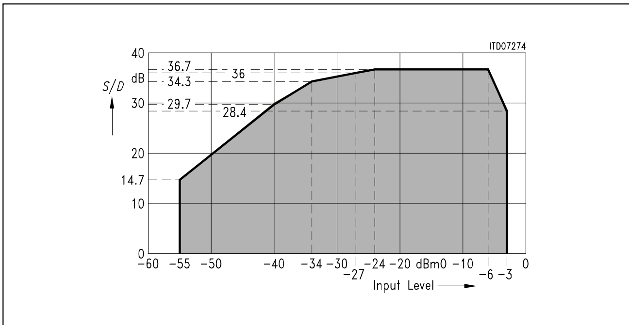
Figure 25 Receive
