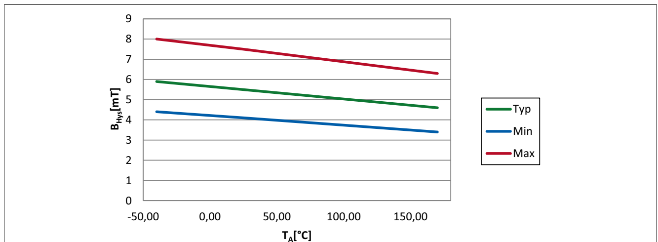
Figure 5-3 Hysteresis ( B_{Hys} ) of the TLE4964-2M over Temperature
