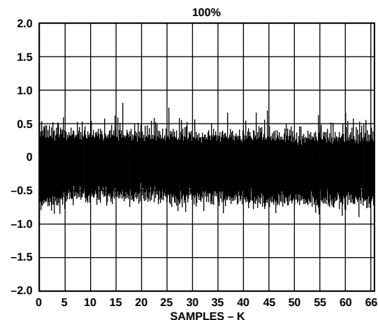
Figure 18. DNL Plot
