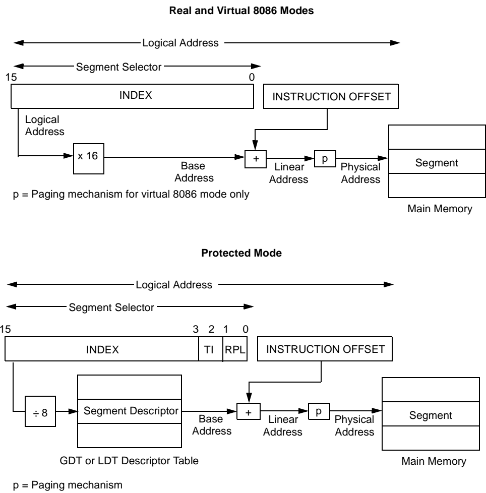
Figure 3-6. Selector Mechanisms
