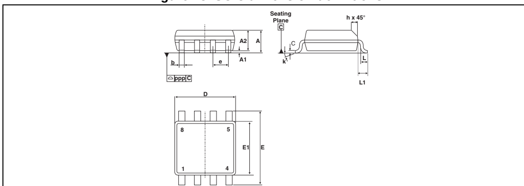
Figure 13. SO-8 dimension definitions
