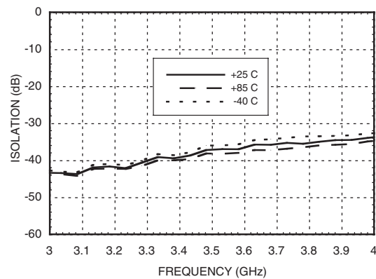
Power Down Isolation vs. Temperature
