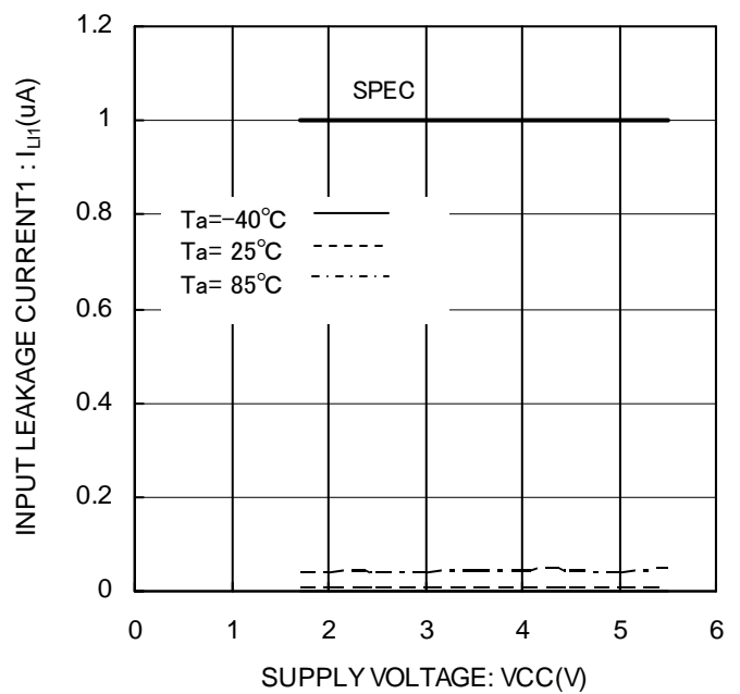
Figure 11. Input leakage current1 I_{IL1} (SK)
