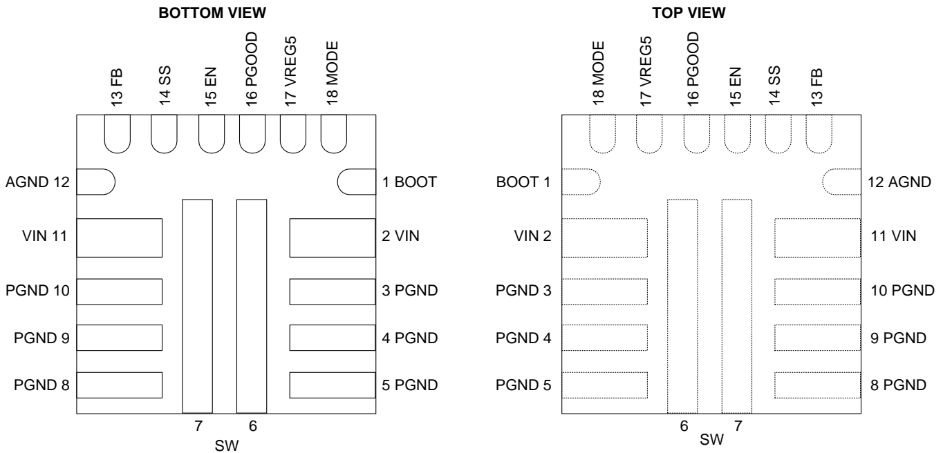
Pin Functions
