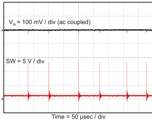
Figure 33. Line Regulation, I_{OUT} = 6\text{ A}
