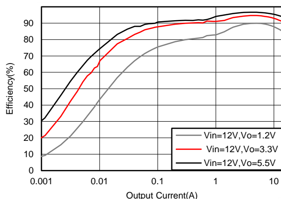
Figure 13. Efficiency, Mode = DCM, F_{SW} = 400\text{kHz}
