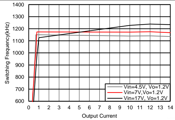
Figure 20. F_{SW} Load Regulation, Mode = DCM, F_{SW} = 1200kHz
