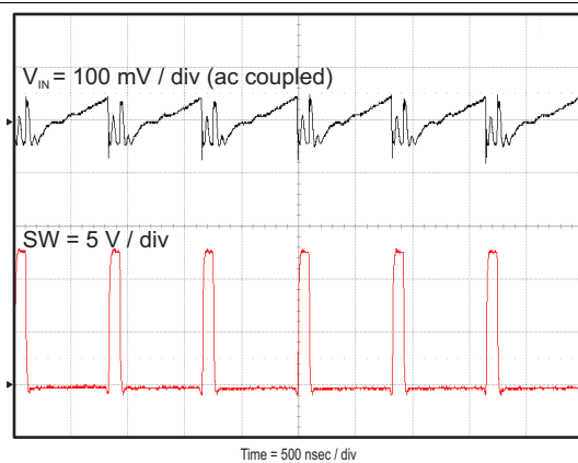
Figure 35. Input Voltage Ripple, I_{OUT} = 10\text{ mA}
