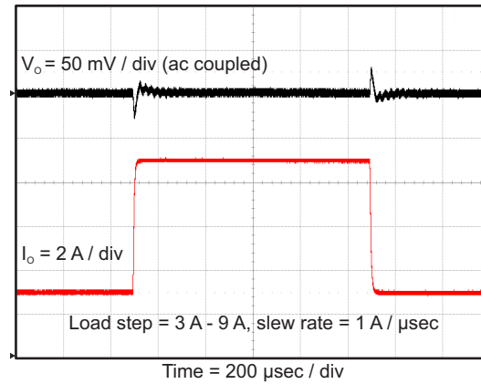
Figure 45. Transient Response
