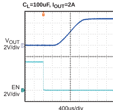
Turn On Delay and Rise Time with 100uF Load
