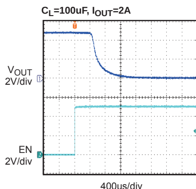
Turn Off Delay and Fall Time with 100uF Load
