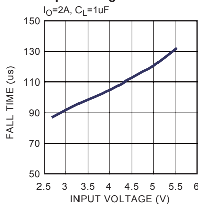
Fall Time vs. Input Voltage I_O=2A , C_L=1\mu F
