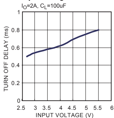
Turn off Delay vs. Input Voltage I_O=2A , C_L=100\mu F
