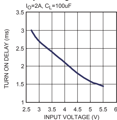
Turn on Delay vs. Input Voltage I_O=2A , C_L=100\mu F
