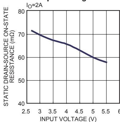
Static Drain-Source On-State Resistance vs. Input Voltage I_O=2A
