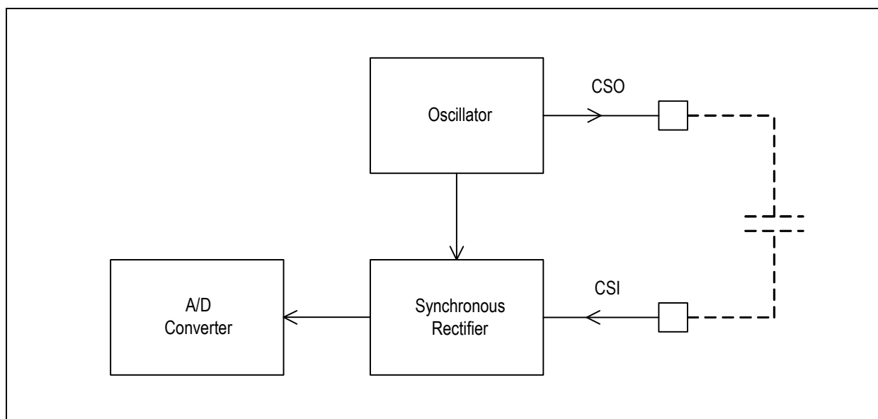
Figure 19: Capacitive Sensor Block Diagram
