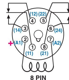
8 PIN
