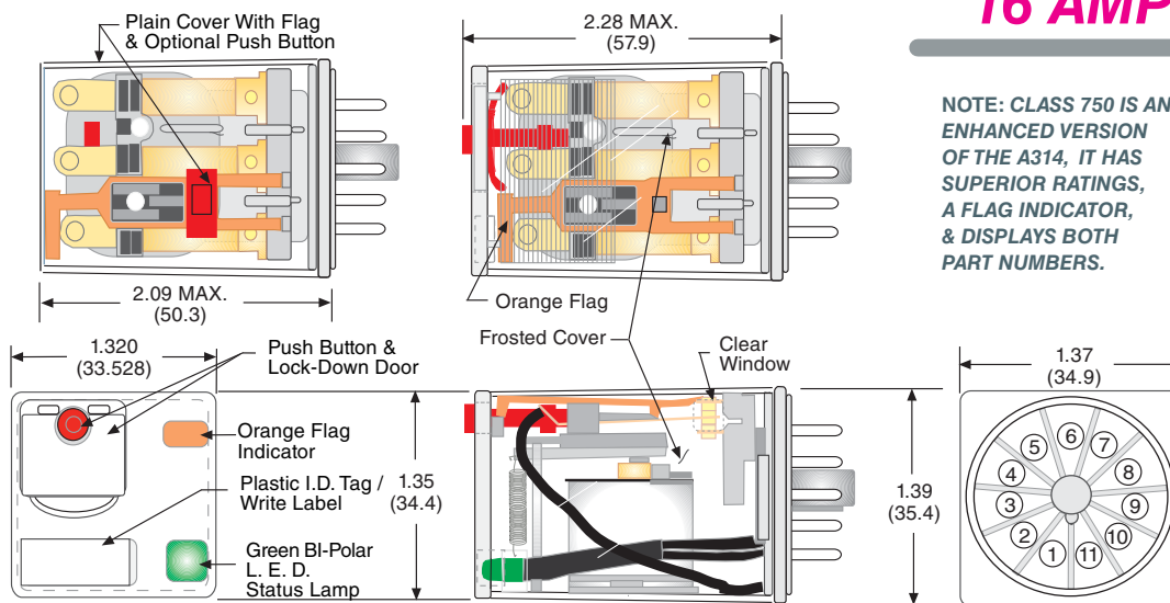
8 PIN OCTAL BASE NOT SHOWN
