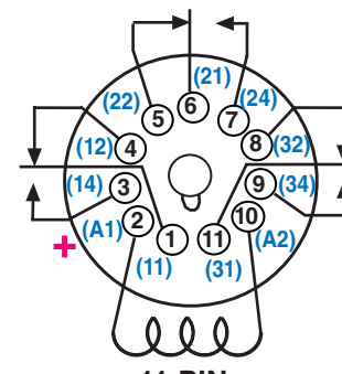
11 PIN
