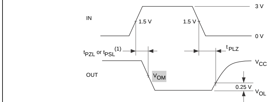
Figure 12: Drive enable and disable times waveforms (pull-up configuration)
