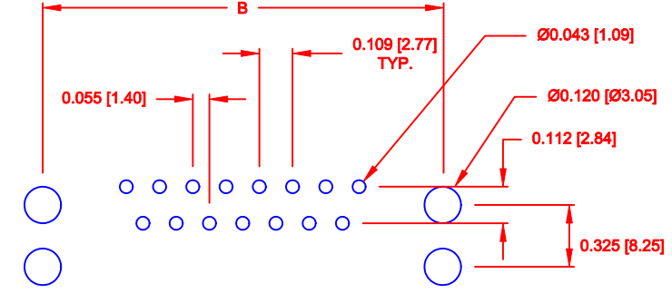
RECOMMENDED PCB LAYOUT SCALE = 2 : 1
