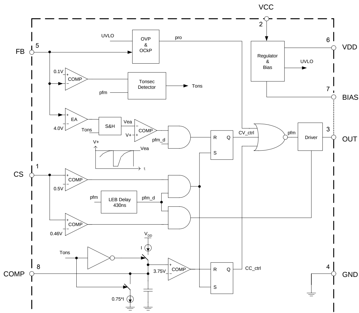
Figure 3. Functional Block Diagram of AP3706
