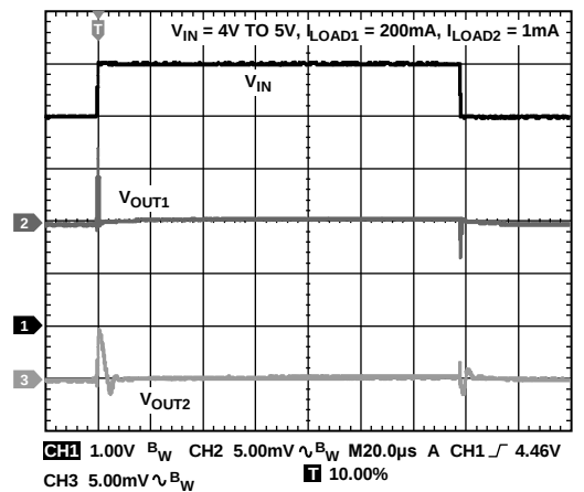
Figure 26. Line Transient Response V_{IN} = 4V to 5V , I_{LOAD1} = 200mA , I_{LOAD2} = 1mA CH1 = V_{IN} , CH2 = V_{OUT1} , CH3 = V_{OUT2}
