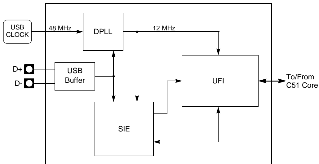
Figure 15-2. USB Connection
