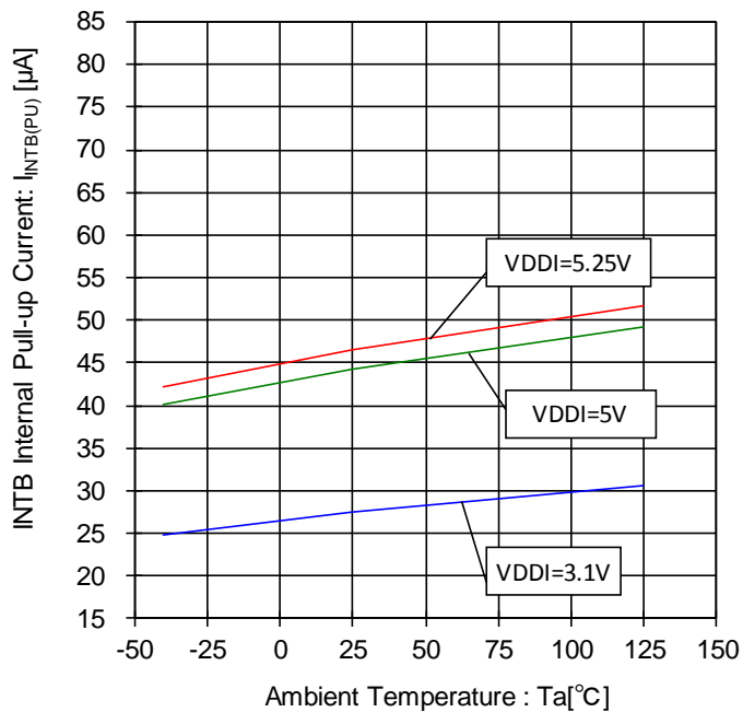
Figure 99. INTB Internal Pull-up Current- Temperature Characteristic
