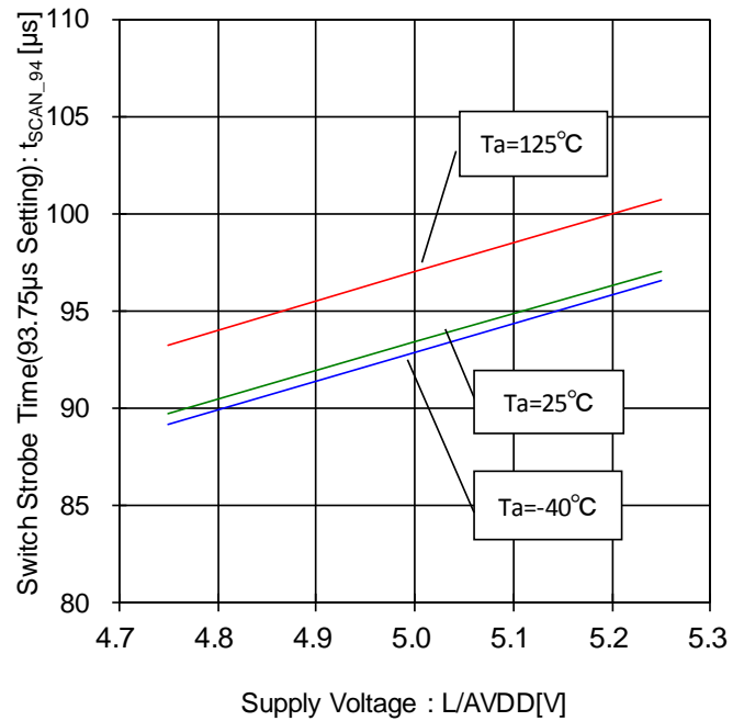
Figure 110. Switch Strobe Time- Voltage Characteristic (93.75μs Setting)
