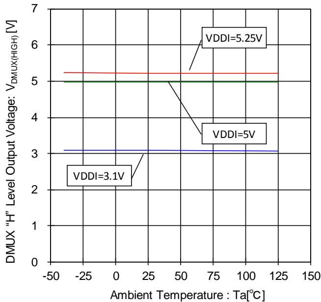
Figure 95. DMUX "H" Level Output Voltage- Temperature Characteristic ( I_{SOURCE}=200\mu\text{A} )
