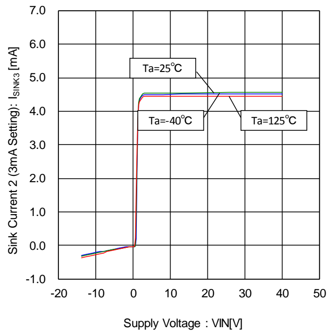
Figure 46. Sink Current 2- Voltage Characteristic (3mA Setting)
