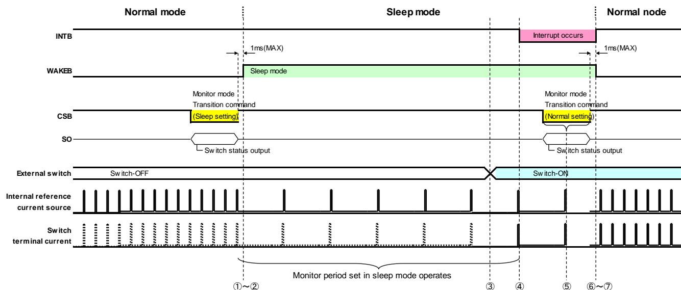
Figure 9. Basic Operation 3
