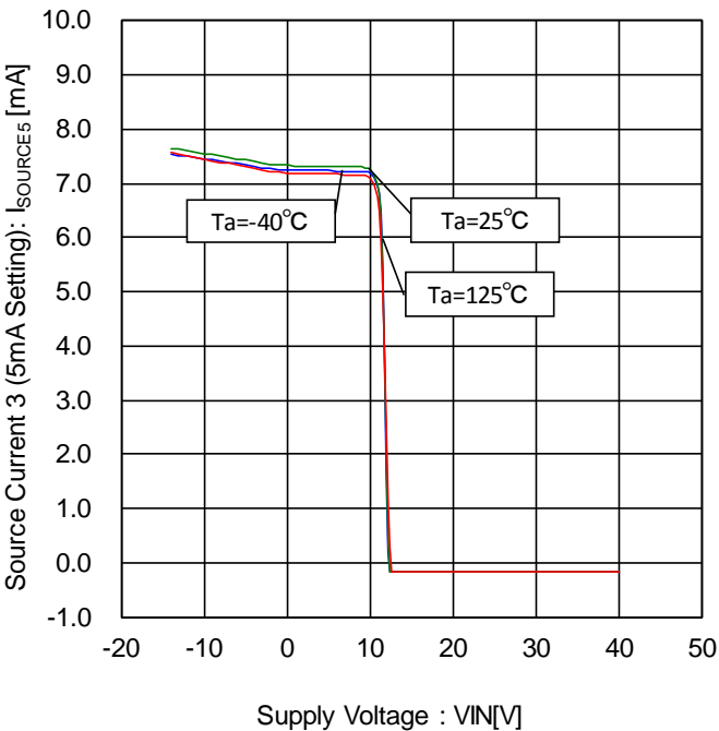
Figure 50. Source Current 3- Voltage Characteristic (5mA Setting)
