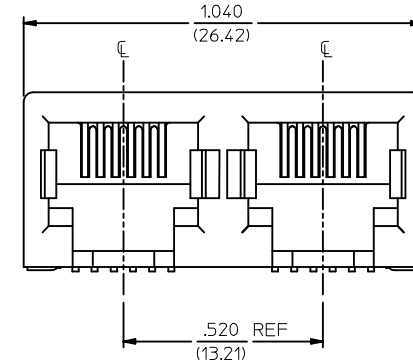
6 CIRCUIT ASSEMBLY
