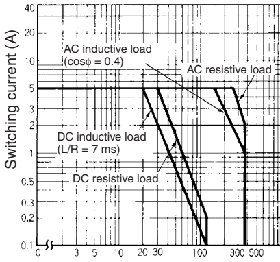
Switching voltage (V)
