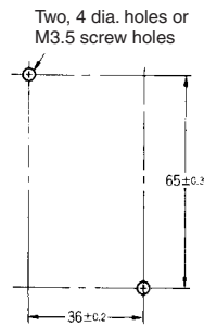
Mounting Holes
