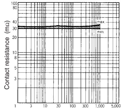
Number of switching operations ( \times 10^4 times)
