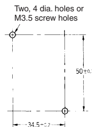
Mounting Holes
