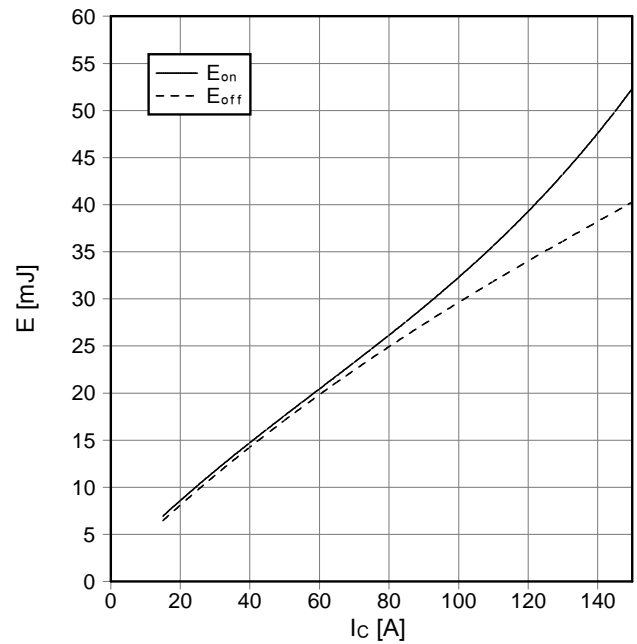
Schaltverluste IGBT-Wechselr. (typisch) switching losses IGBT-inverter (typical) E_{on} = f(I_C), E_{off} = f(I_C) V_{GE} = \pm 15\text{ V}, R_{Gon} = 6,8\ \Omega, R_{Goff} = 6,8\ \Omega, V_{CE} = 900\text{ V}, T_{vj} = 125^\circ\text{C}
