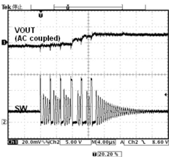
Figure 7. SW and VOUT waveforms at SLLM (Light load)
