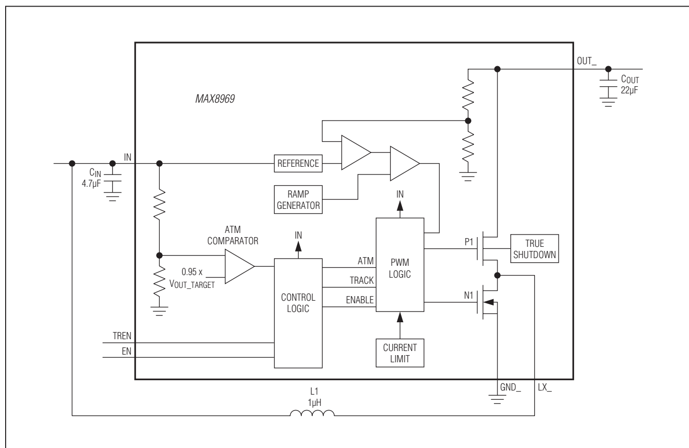
Figure 1. Functional Diagram
