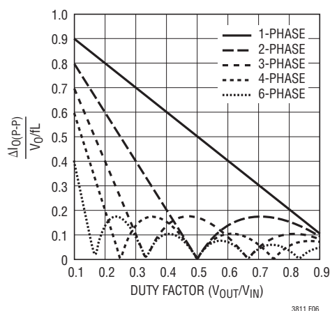
Figure 6. Normalized Peak Output Current vs Duty factor [ I_{RMS} \approx 0.3(\Delta I_{O(P-P)}) ]
