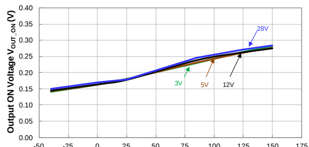
Temperature (°C) Output ON Voltage vs Temperature
