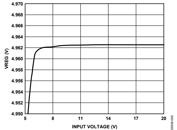
Figure 9. VREG vs. Input Voltage, 10 mA Load
