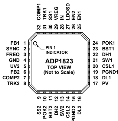
Figure 3. Pin Configuration
