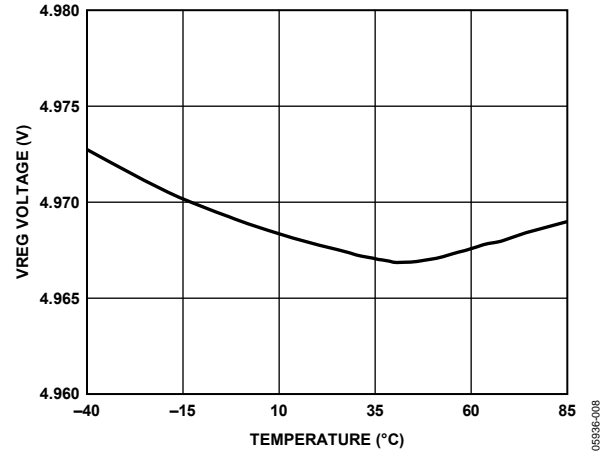
Figure 8. VREG Voltage vs. Temperature
