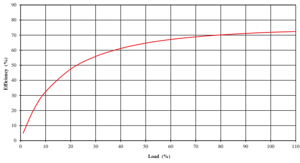
NXE2S1212MC
