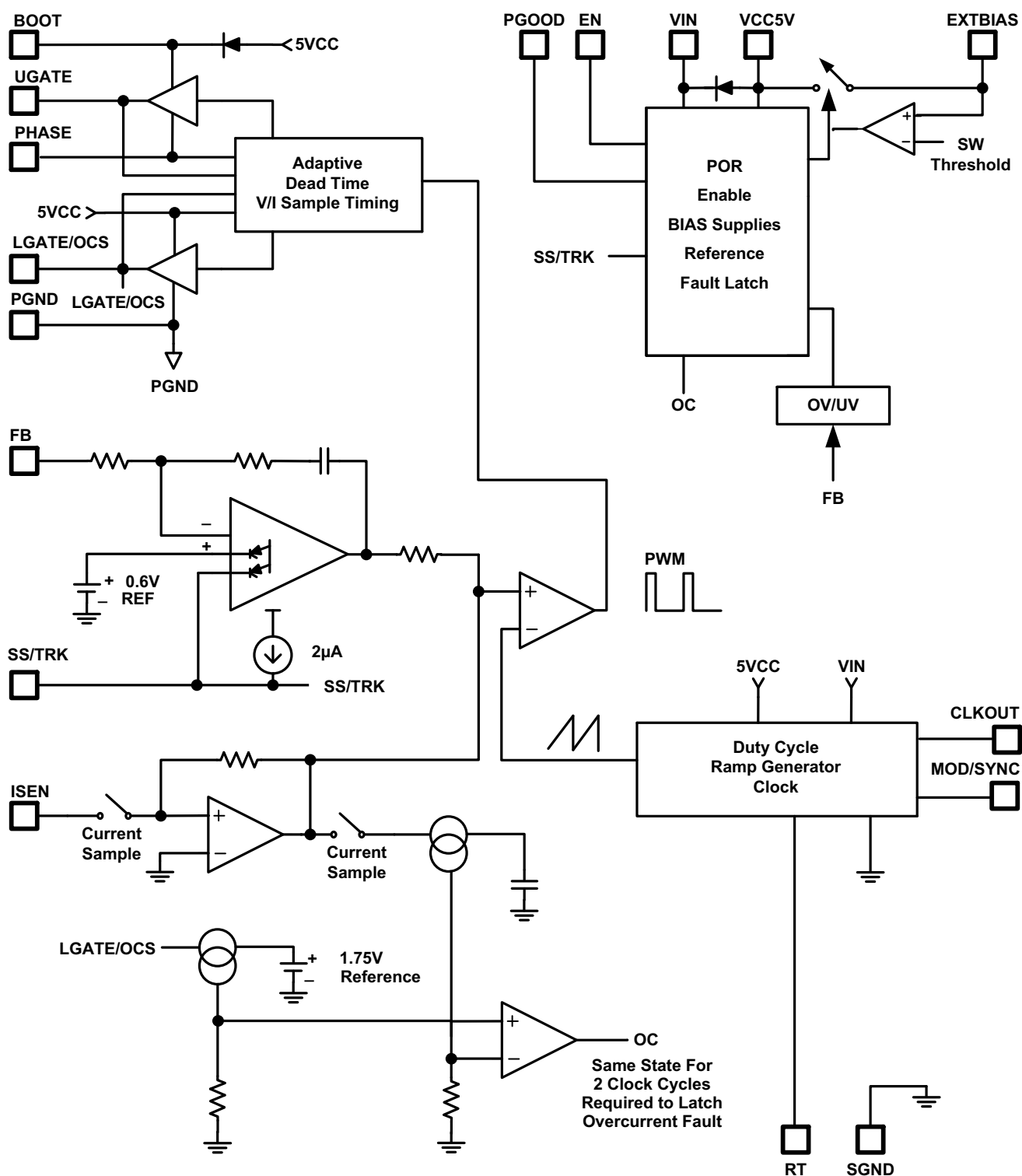
Figure 3. Block Diagram
