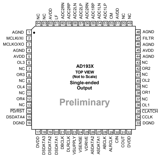
Figure 22. Single-ended Output 64-Lead LQFP (AD1935)
