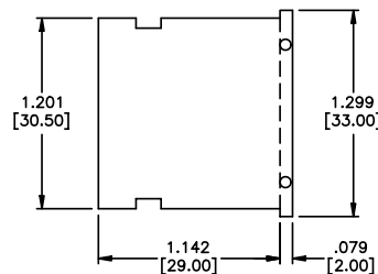
DPS910A2 Spacer
