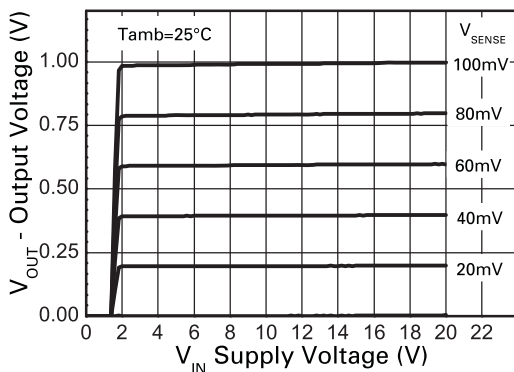
Transfer Characteristic
