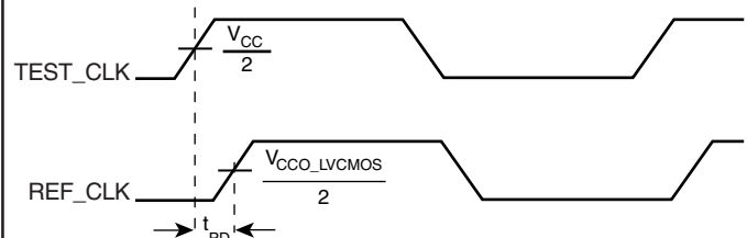
PROPAGATION DELAY
