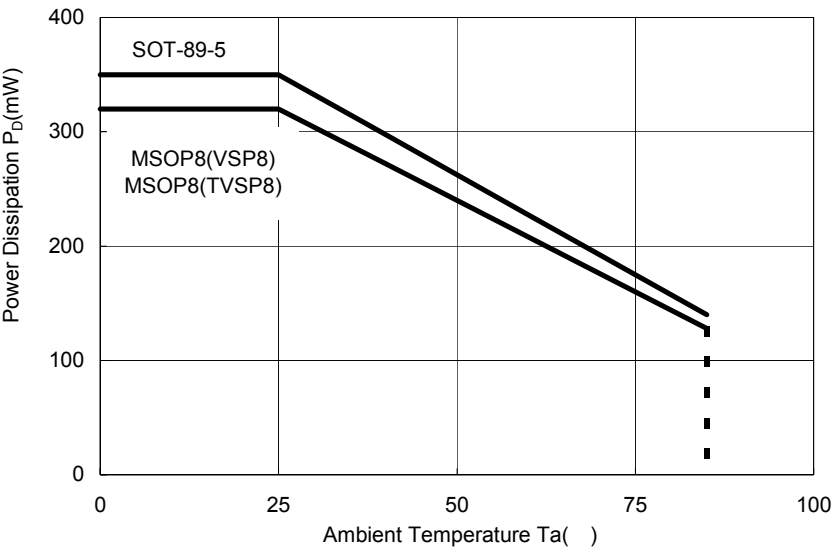
NJM2370 Power Dissipation (Topr=-40 ~ +85 ,Tj=125 )
